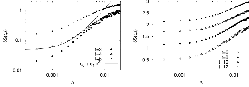
Figure 6: \delta S_B(t, \Delta) with \epsilon = 10^{-4} as a function of \Delta for small values of t (left panel) and large values of t (right panel). In the left panel the line shows the expected behavior c_0 + c_1 \Delta^2 while in the right panel \delta S_B(t, \Delta) shows a weak dependence on \Delta for \Delta \rightarrow 0 .
