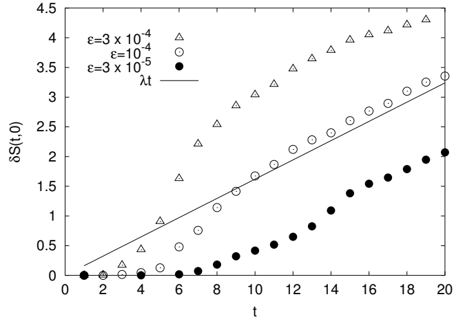
Figure 7: Extrapolation for \Delta \rightarrow 0 of the curves \delta S_B(t, \Delta) as a function of t for various values of \epsilon .
