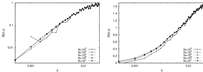
Figure 4: Comparison of Boltzmann entropy growth as a function of \Delta at fixed time, plotted for different values of N . Parameters are k = 0.017 , \epsilon = 0 and N_S = 1000 ; t = 3 in the left picture and t = 9 in the right one. Small numerical differences between these figures and Fig. 3 are due to a different realization of the obstacles positions.
