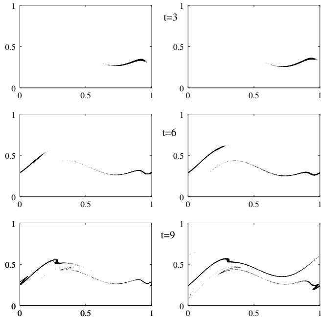
Figure 8: Snapshots of the evolution of the system in the single-particle projection of the phase space in the non-interacting case (left), and in the interacting case with \epsilon = 10^{-4} (right) and M = 100 , at increasing times from top to bottom, as indicated in the figure.
