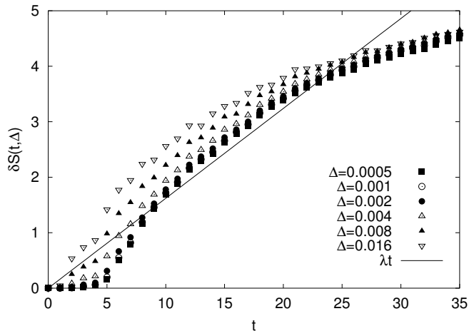
Figure 5: \delta S_B(t, \Delta) with \epsilon = 10^{-4} as a function of t for different values of \Delta . The straight line slope equals the Lyapunov exponent.
