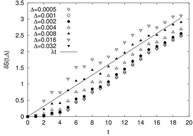
Figure 9: Numerical simulation of N = 10^7 independent particles evolving according to (23) with \epsilon_{eq} = 10^{-4} . Notice the similar qualitative behavior observed in Fig.(5).
