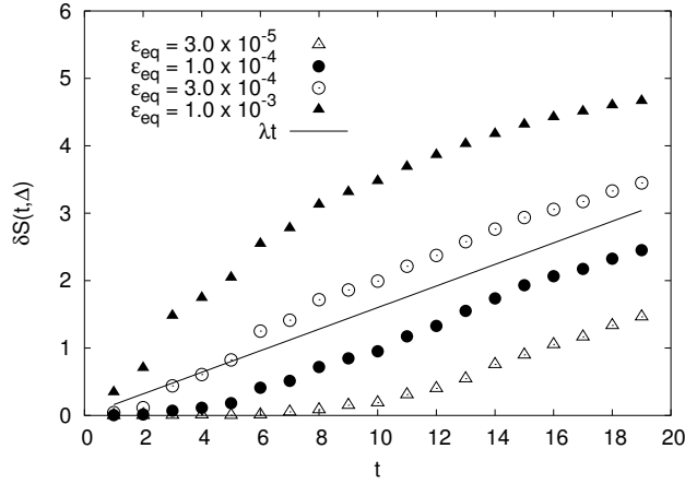
Figure 10: Extrapolation for \Delta \rightarrow 0 of the curves \delta S_B(t, \Delta) as a function of t for various values of \epsilon_{eq} . Notice that the extrapolated curves are qualitatively similar to the interacting case (cf. Fig. 7).
