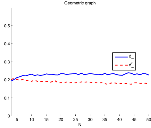
Fig. 3. d_\infty^r and d_\infty for random geometric graphs, averaged over 25 realizations of the initial condition and 18 of the graphs, for each N . The plot assumes \sigma^2 = 1/12 .
