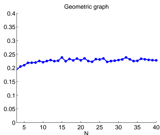
Fig. 1. Performance of the random geometric graph. Since the graph itself is random, the plot of d_\infty(P) comes from averaging over realizations of both the graph and the initial condition.
