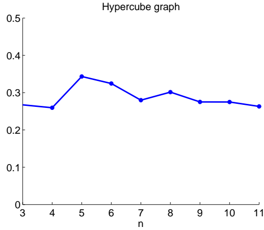
Fig. 2. Performance of the n -dimensional hypercube graph (of order N = 2^n ).
